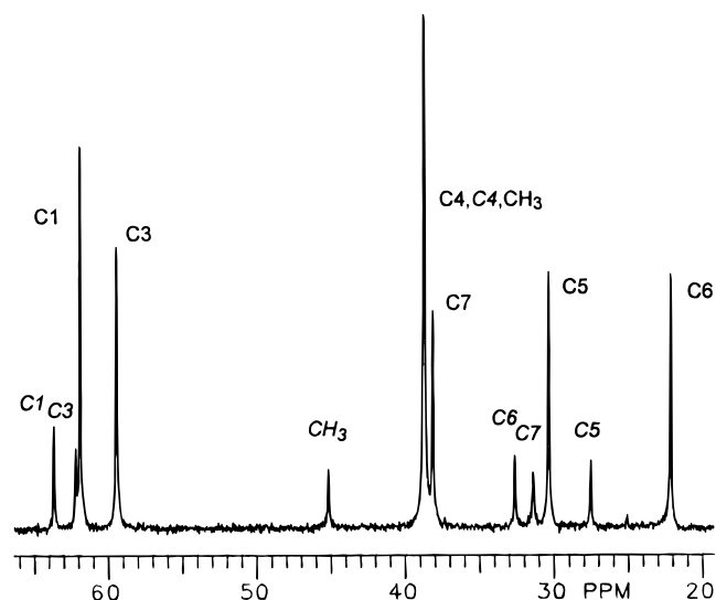
Figure 1. The 126 K, 75.43 MHz ^{13}\text{C}\{^1\text{H}\} NMR spectrum of 2 . The major isomer is 2-endo ; signal assignments for 2-exo are indicated by italics.
