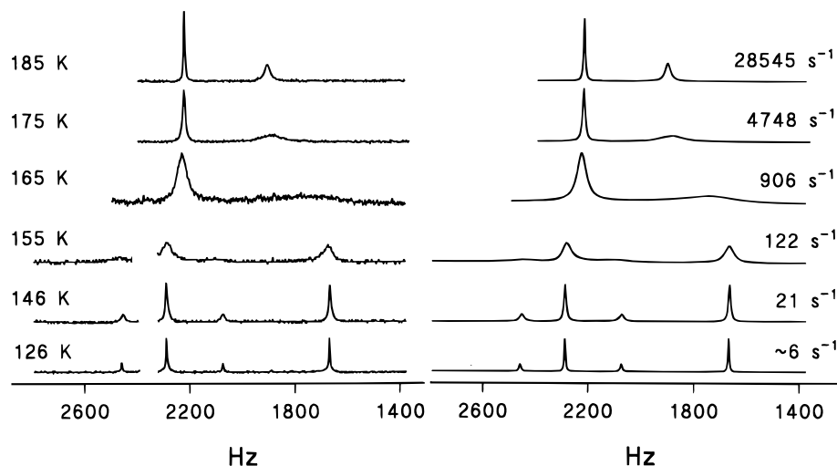
Figure 2. Experimental 75.43 MHz ^{13}\text{C}\{^1\text{H}\} NMR spectra of the C5,C6 region of 2 in the left column and DNMR5 theoretical simulations in the right column. The experimental spectra were digitized in the DNMR5 program, and the C7 signal of 2-exo has been removed for clarity from the three lowest temperature spectra.
