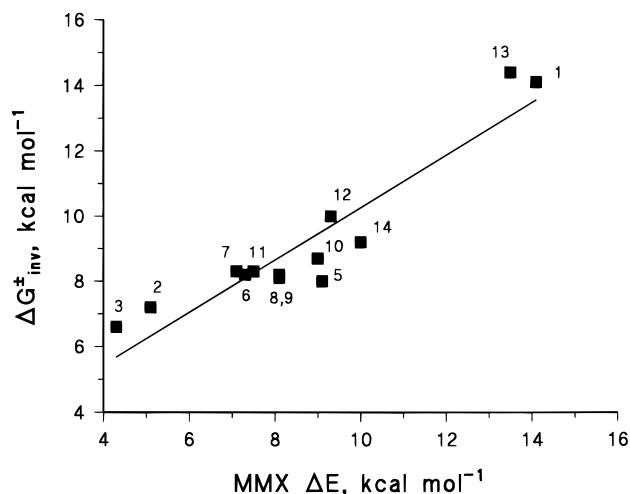
Figure 3. Plot of inversion-dominated amine exchange barriers, \Delta G^\ddagger , vs MMX calculation of energy change, \Delta E , between pyramidal and planar forms.
